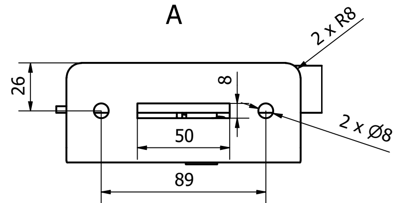
VIEW A
